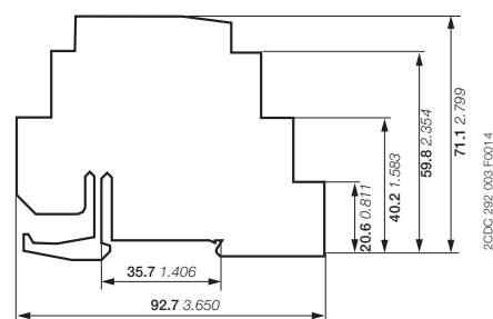
Separator for CR-S
