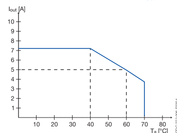
Temperature curve at U_{out} = 24 V DC
