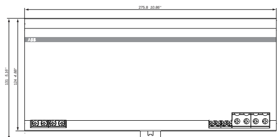
CP-T 24/40.0, CP-T 48/20.0
