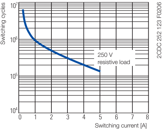
Contact lifetime
