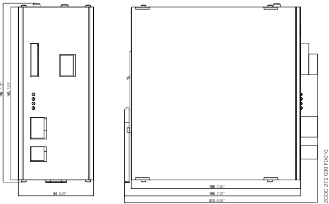
CP-B 24/20.0
