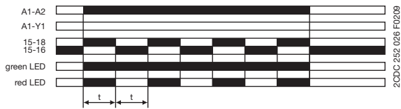
t = adjusted flashing time
