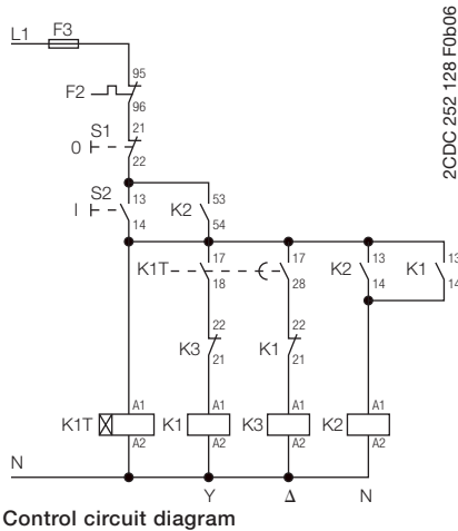
Control circuit diagram
