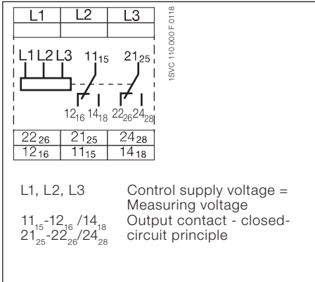
Connection diagram CM-MPS.31, CM-MPS.41, CM-MPS.43
