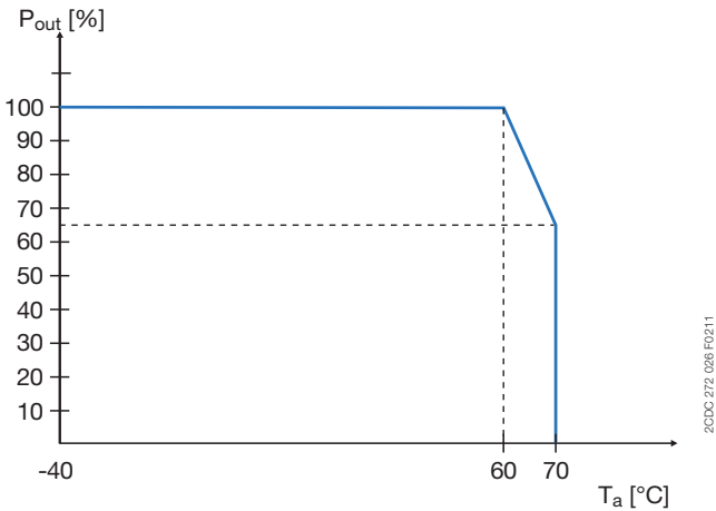
CP-T 24/40.0, CP-T 48/20.0
