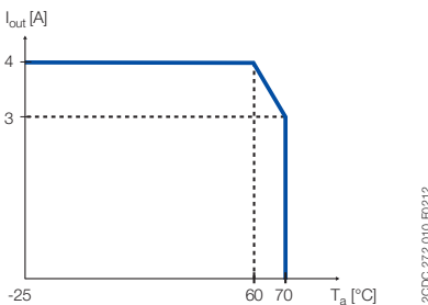
Characteristic curve of temperature at rated load
