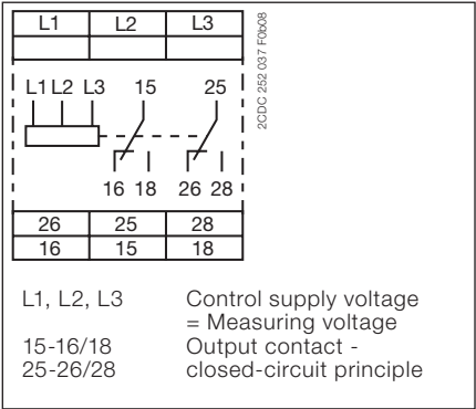
Connection diagram CM-MPS.11, CM-MPS.21, CM-MPS.23
