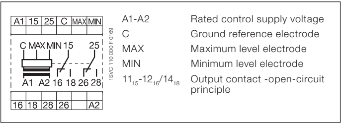
Connection diagram CM-ENN
