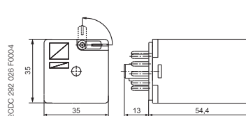
CR-U with 3 c/o contacts
