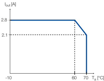
Characteristic curve of temperature at rated load
