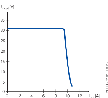
Output behaviour
