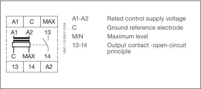
Connection diagram CM-ENN
