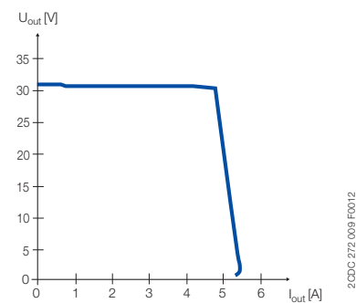
Output behaviour
