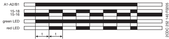
t = adjusted flashing time
