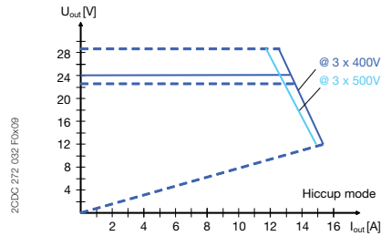
CP-T 24/10.0
