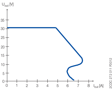
Output behaviour
