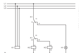
Control circuit diagram (K1 = CM-MPS.43 or CM-MPN.xx)
