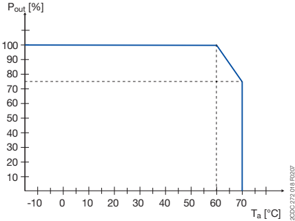
Characteristic curve of temperature at rated output voltage
