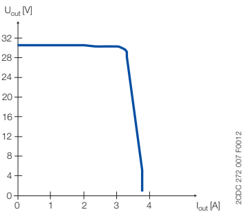
Output behaviour
