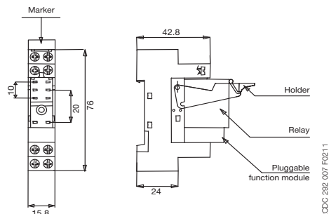
CR-PSS - screw connection
