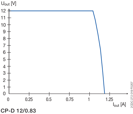
Characteristic curve of output at Ta = 25 °C
