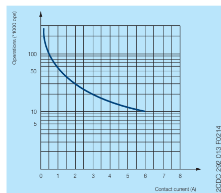
Endurance curve
