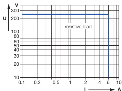
AC load (resistive)
