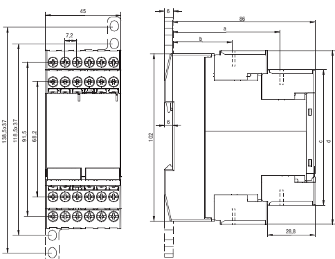
C512/C513 45 mm
