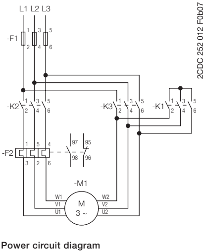
Power circuit diagram
