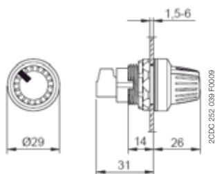
CT-S time relay
