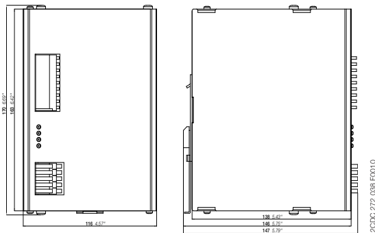
CP-B 24/10.0
