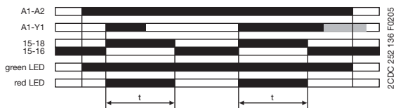
t = adjusted pulse time
