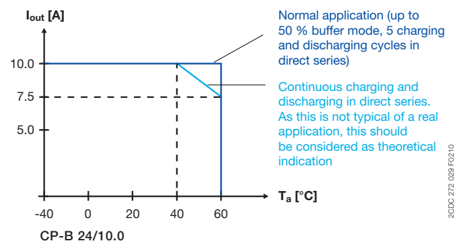
Caracteristic curve of the temperature at rated load
