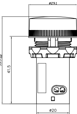
Buzzer
