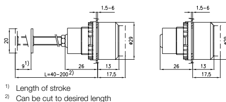
Reset pushbutton
