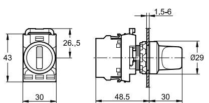
Selector switch
