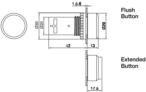
Pushbutton
