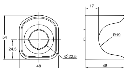
Emergency stop shroud Modular range
