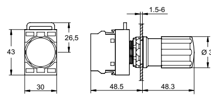
Emergency stop type MPE
