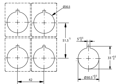
Drilling plan for 30 mm adaptor
