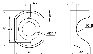
Emergency stop shroud Compact range
