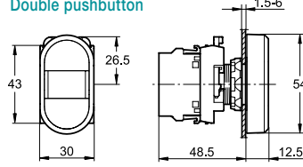
Double pushbutton
