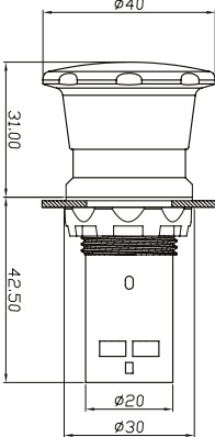
Mushroom
