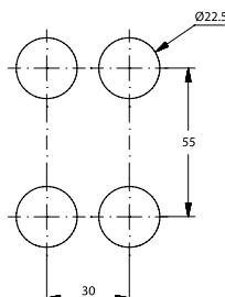
Drilling plan for double pushbutton
