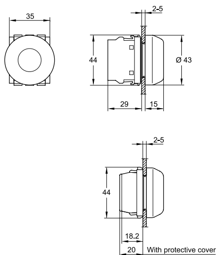
Heavy duty pushbutton
