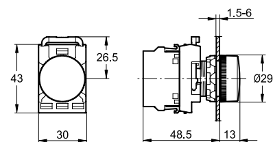
Pilot light
