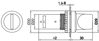
Selector switch
