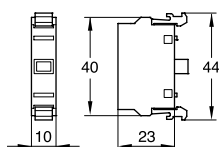
Contact block (for front mounting)
