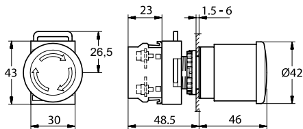
Emergency stop type MPM
