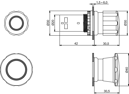
Emergency stop CE3P/CE4P (Pull release)
