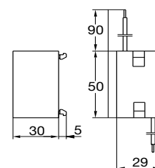
Transformer block
