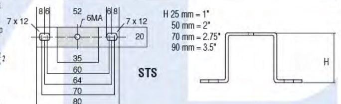
6 mm screws included ST and STS screw size 6 mm All dimensions shown are in mm
