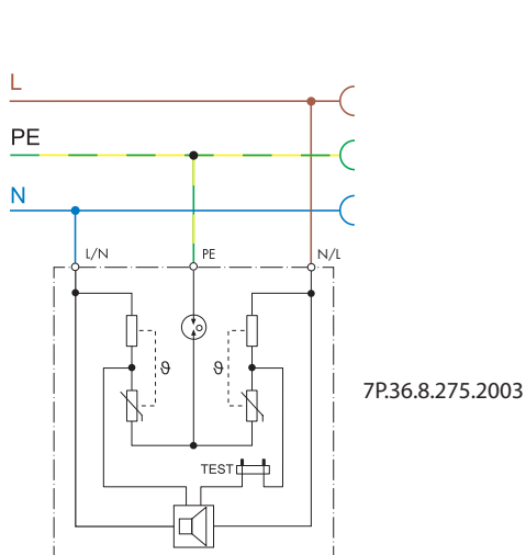
TT or TN-S SINGLE PHASE SYSTEM - INCORPORATED IN SOCKET OUTLET
