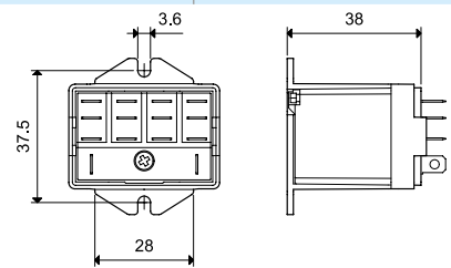
056.45 with relay
