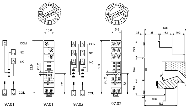
97.02 + 46.52 + 097.01 + 86.30
