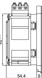
AC version
