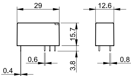
Types 41.31/52/61
