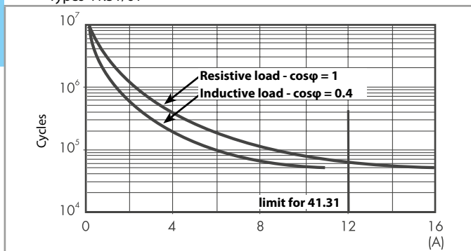
F 41 - Electrical life (AC) v contact current (bistable)
