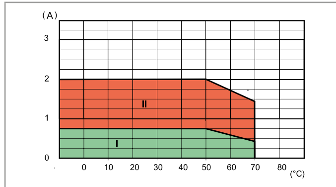
L 34 - Output AC current v ambient temperature
