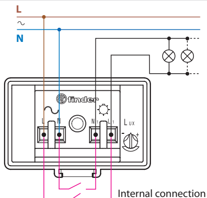
Type 10.32
