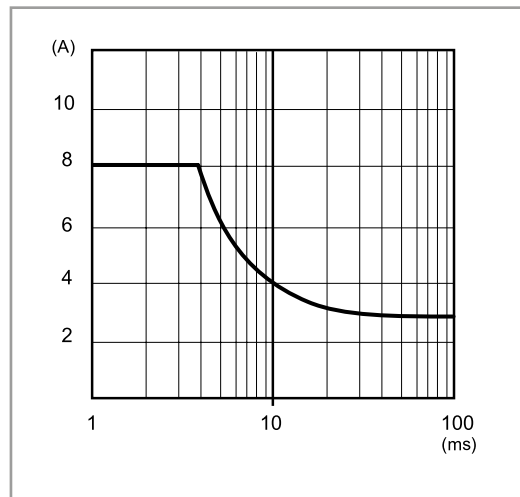
P78-5 Output peak current v time (78.61)
