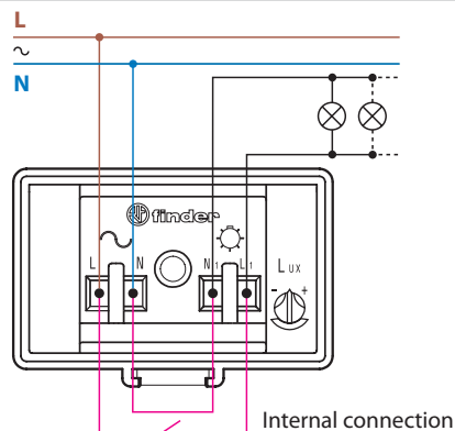
Type 10.41
