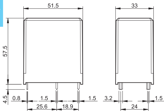
Type 67.22
