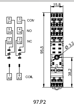
97.P2
