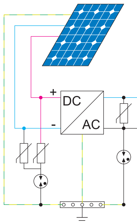
Figure 10: Example of a photovoltaic system located on a building without LPS, protected on the DC side by an SPD with U_{OCSTC} = 420\text{ V} , and on the AC side by a 7P.22, specific for TT systems.
