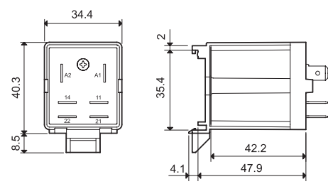
065.07 with relay
