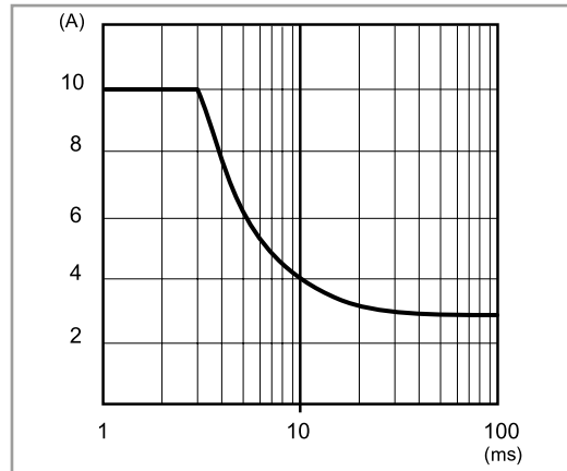
P78-4 Output peak current v time (78.50/51)
