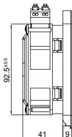
DC version
