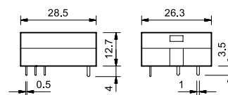
Type 40.11 (page 5)
